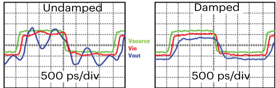
Figure 5. Adding a resistor to a probe tip can overcome resonance from long probe connections, reduce ringing and overshoot. However, it will not prevent bandwidth limiting caused by the added leads.
